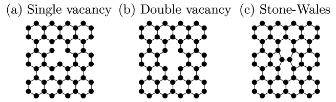
Figure 1 Defects in graphene nanoribbons: (a) single vacancy, breaking the degeneracy between the two sublattices; (b) double vacancy which equally affects both sublattices; (c) Stone–Wales deformation: four hexagons are replaced by pairs of pentagons and heptagons.
