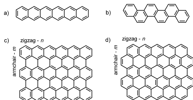
Figure 1. Structures investigated: a) n -acene, b) n -phenacene, c) ( m , n , z ) periacene, and d) ( m , n , z ) circumacene.
