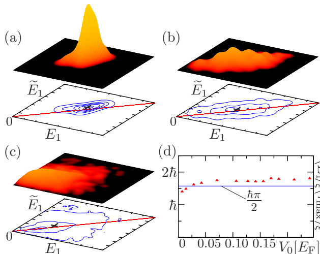
Fig. 3: (Color online) Smoothed distribution of (E_1, \tilde{E}_1) pairs for three different strengths of the disorder potential, (a) V_0/E_F = 0.007 , (b) 0.03, (c) 0.24 (500 realizations of disorder were used). Black crosses in the contour plot mark the mean value of the distribution. A perfect (E_1, \tilde{E}_1) correlation would correspond to a non-vanishing density only along the diagonal (drawn in the contour plot as guide to the eye). (d) Product of the mean gap size \langle E_1 \rangle_\xi and the mean of the maximum Wigner-Smith delay time \langle \tau_{\max} \rangle_\xi as a function of disorder strength. The constant value \hbar\pi/2 (predicted by eq. (5)) is shown for comparison.
