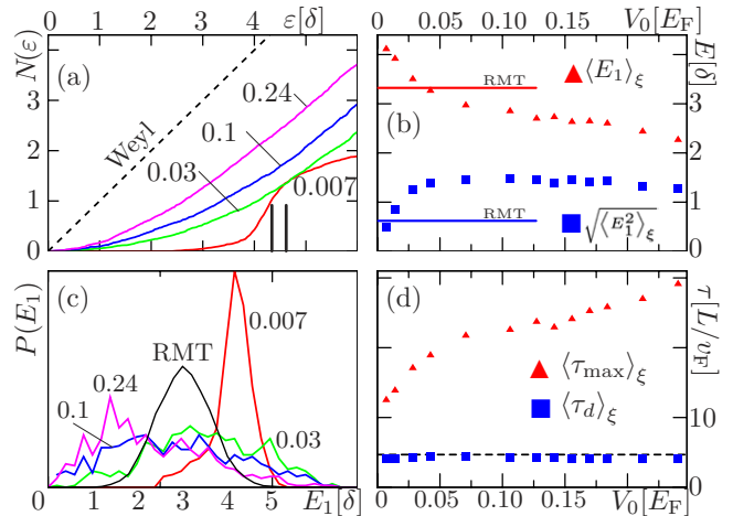
Fig. 2: (Color online) (a) Disorder-averaged state counting function, \langle N(\varepsilon) \rangle_\xi , for four different disorder strengths V_0/E_F = 0.007, 0.03, 0.1 and 0.24 (colored solid lines) and Weyl estimate (black dashed line). The two lowest-energy eigenvalues of the disorder-free system are marked by vertical bars. (b) Evolution of the mean gap \langle E_1 \rangle_\xi (red triangles) and the root mean square deviation (blue squares) as a function of disorder strength V_0 (in units of E_F ). Horizontal lines mark the RMT predictions. (c) Statistical distribution of the lowest eigenvalue E_1 for four disorder strengths V_0 (colored lines) compared with the RMT distribution (black line). (d) Dependence of the Wigner-Smith delay times on disorder strength V_0 . Both the mean delay time, i.e. , the dwell time \langle \tau_d \rangle_\xi (blue squares), and the maximum delay times \langle \tau_{\max} \rangle_\xi (red triangles) are shown. The black dashed line shows the estimate \langle \tau_d \rangle_\xi = 2\pi/N\delta' from [32].
