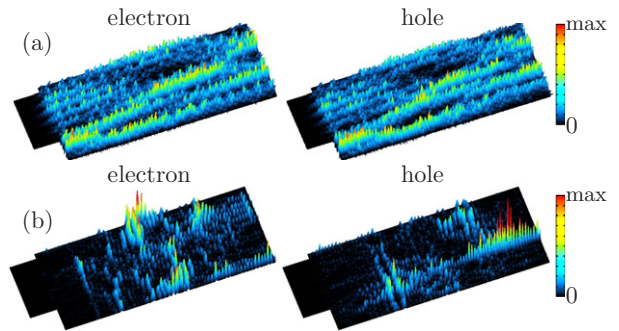
Fig. 4: (Color online) Electron and hole probability densities of the lowest Andreev eigenstate at (a) zero disorder potential, (b) finite disorder strength V_0/E_F = 0.15 (one disorder realization).
